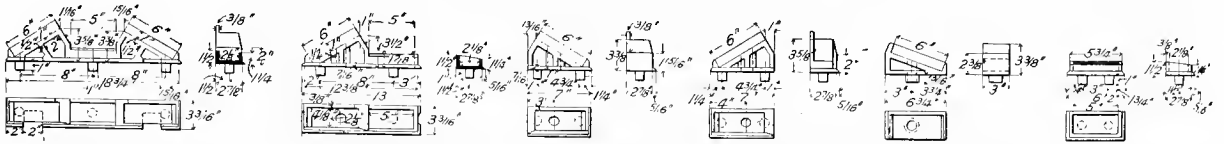
Figs. 696-698. Double Brace and Post Casting (4). Figs. 699-701. Single Brace and Post Casting (4). Figs. 702-704. Side Brace Casting at Corner Post (4). Figs. 705-707. Side Brace Casting at Door Post (4). Figs. 708-710. End Brace Casting (5). Figs. 711-713. Side Post Socket Casting (4).
